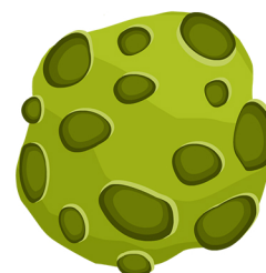
Asteroida
